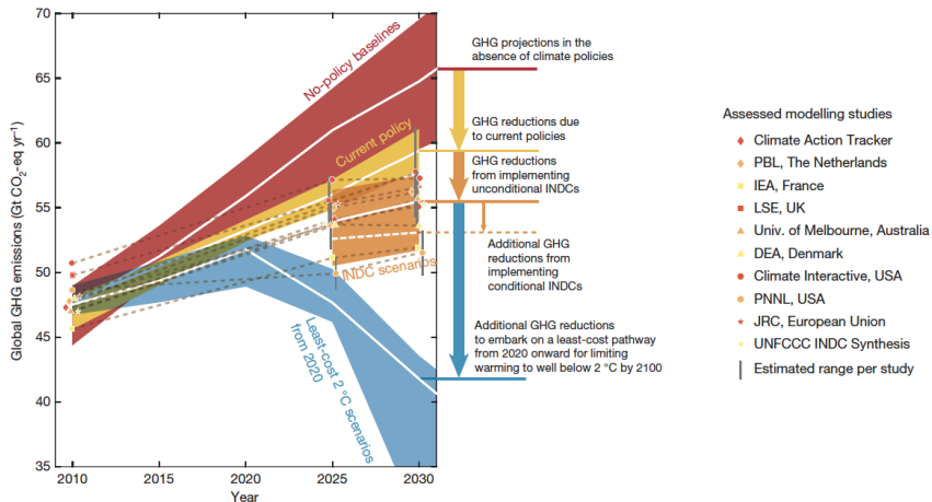
Figure 18: Global GHG emissions trends under different scenarios. After Rogelj et al. (2016)
