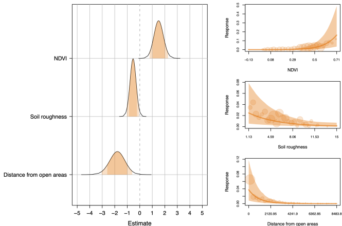
Figure 14: Estimated fixed effects of environmental variables on the probability of occurrence of C. marthae . After Gargano et al. (2025)
